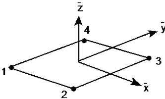
Local coordinate system for GCON defined shell elements
