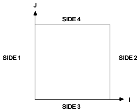
2Dimensional models
