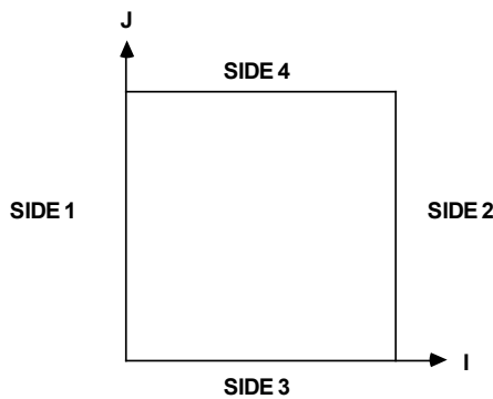
2Dimensional models
