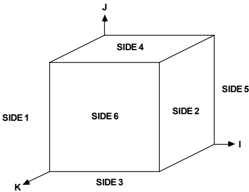
3Dimensional models
