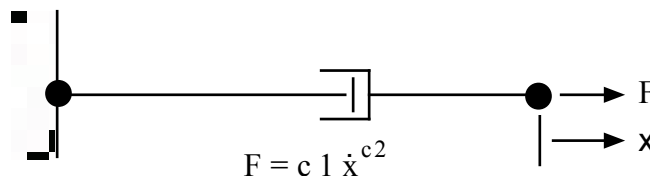
Viscous element of linetype = VISC
