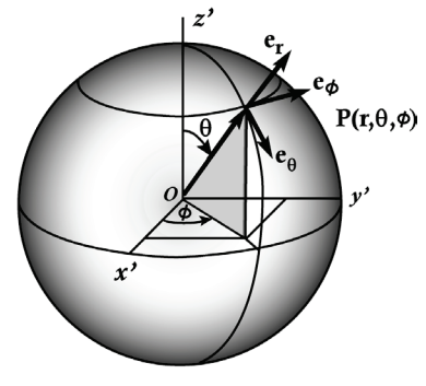
(c) Spherical
