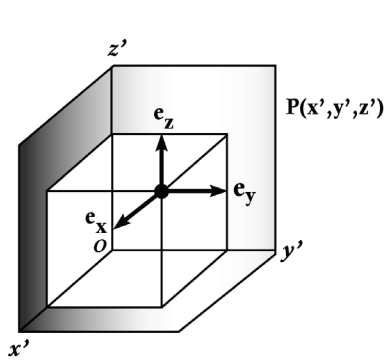
(a) Cartesian
