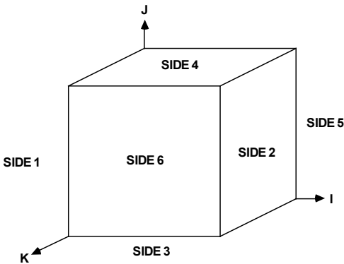
3D models
