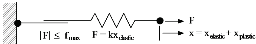
Spring element of linetype = SPR2
