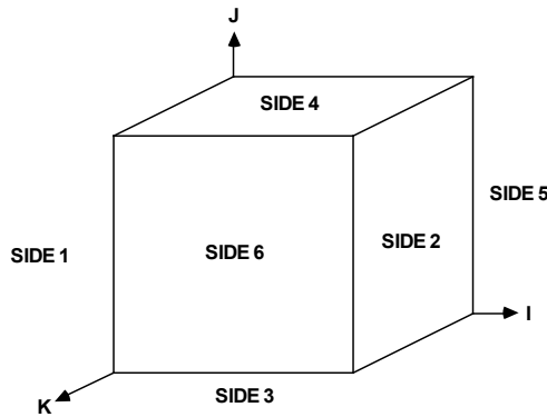
3Dimensional models
