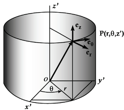
(b) Cylindrical
