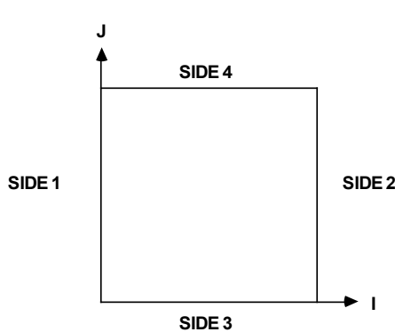
2D models
