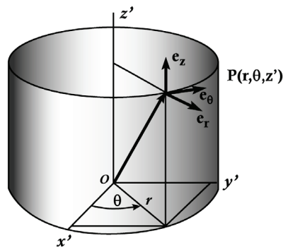
(b) Cylindrical
