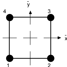
Local coordinate system for SNGL defined membrane elements
